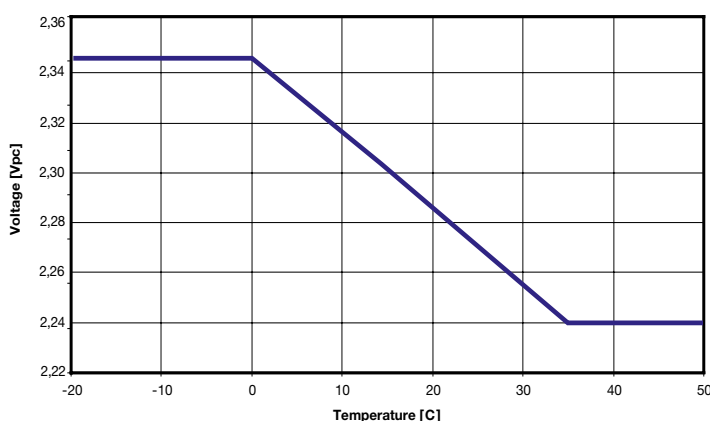
Fig. 5: Sprinter PP; charging voltage vs. temperature
