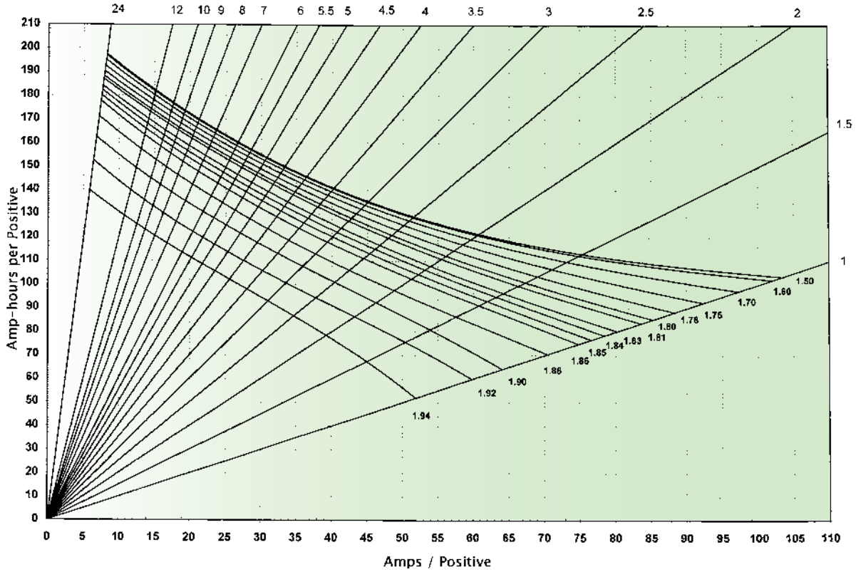
Absolyte ® GX Performance Curves - Constant Current, 1 to 24 hours
