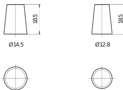
Positive Terminal
